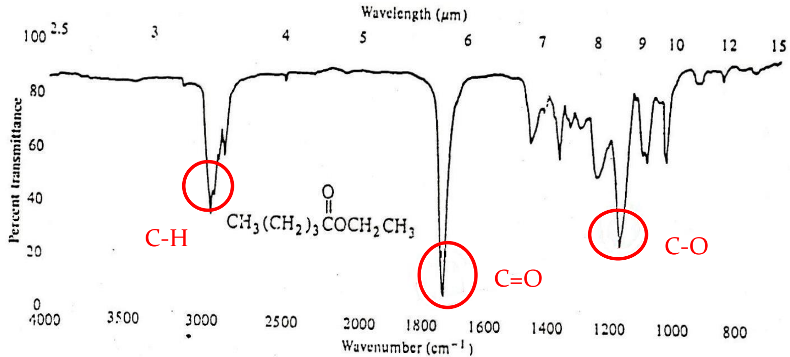
Ethyl pentanoate IR Spectrum
