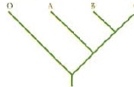
(A) Phylogeny based on sequence of gene 1
