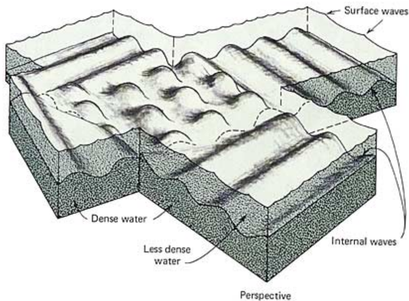
Figure 2: Internal waves at interface between two layers of water of different densities. One is dense (the lower one), the other one is less dense (the upper one). ( Oceanography , Gross, p. 204.)
