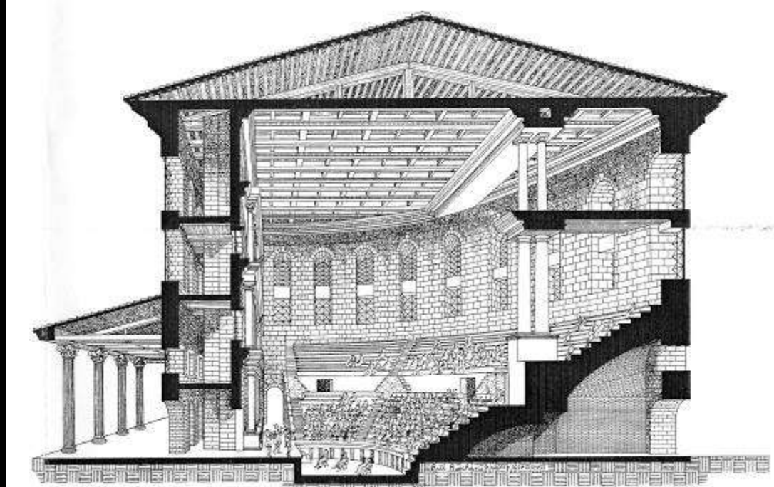
Fig. 15. Restored drawing of stage building of Bouleuterion
