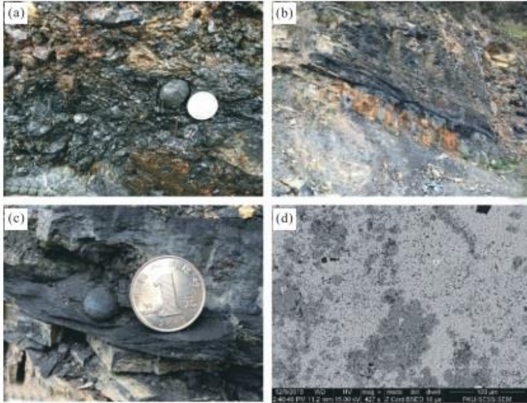
Figure 3. Field photographs of the basal Niutitang Formation and SEM photomicrograph of phosphorite nodule. (a) Phosphorite nodules in the basal Niutitang Formation (the Zhalagou Section); (b) unconformity between the Ediacaran Dengying Formation and the Early Cambrian black shale of the Niutitang Formation in the Songlin Section; (c) phosphorite nodules in the base of the Niutitang Formation; (d) SEM photomicrograph of the phosphorite nodule collected from the Songtao section. P. phosphate; Q. quartz.
