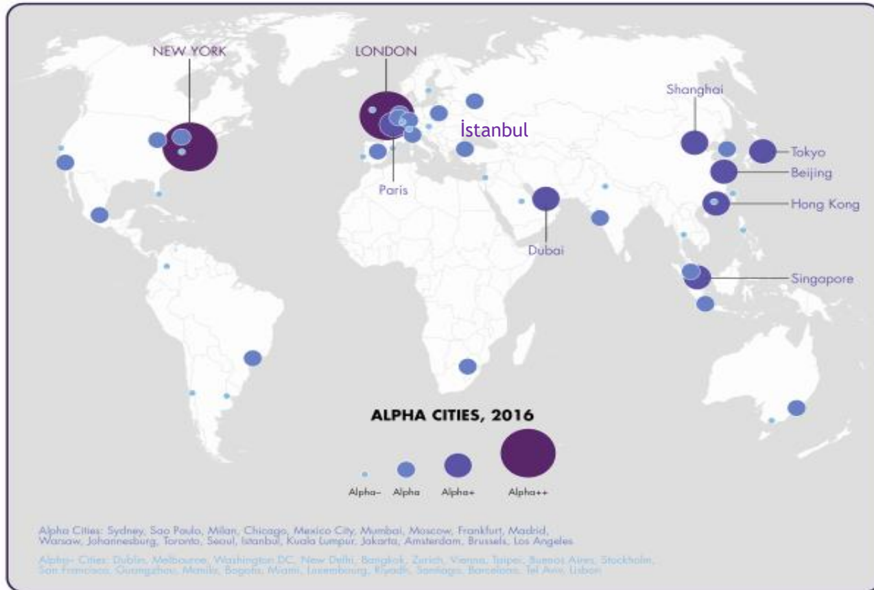
Figure 1: Alpha Cities by Category
