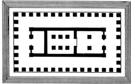
Abb. 22 Magnesia, Artemistempel
