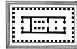
Abb. 22 Magnesia, Artemistempel
