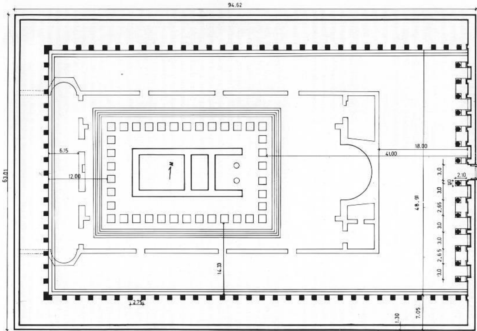
THE SANCTUARY OF APHRODITE 0 5 10 m. Architectural
