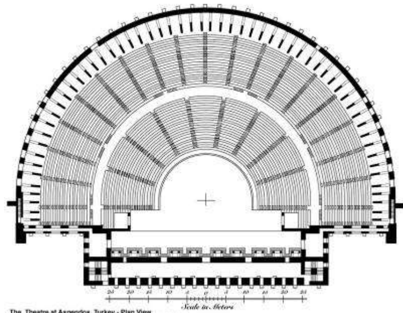
The Theatre at Aspendos, Turkey - Plan View Date of Construction: ca. 160 AD - Seating Capacity: 15,000 Theatron: 99w X 73 meters - 325w X 240 feet / Orchestra: 24w X 20 meters - 79w X 66 feet / Stage: 49.5w X 7 meters - 162w X 23 feet (approximate measurements based on reconstruction drawing)
