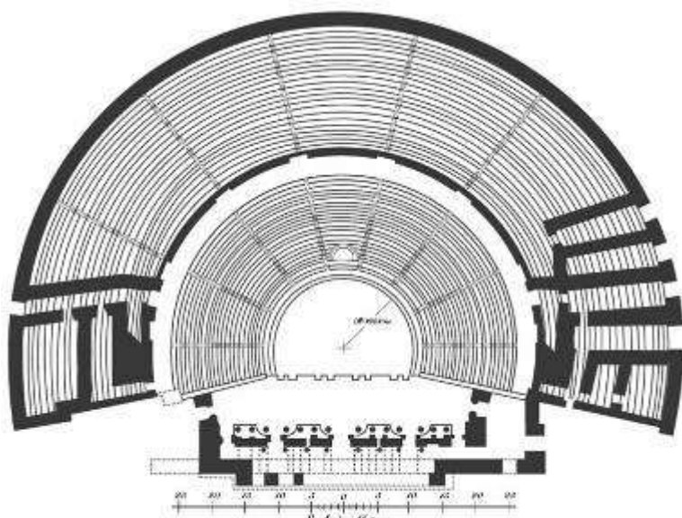
The Greco-Roman Theatre at Hierapolis - Plan View
