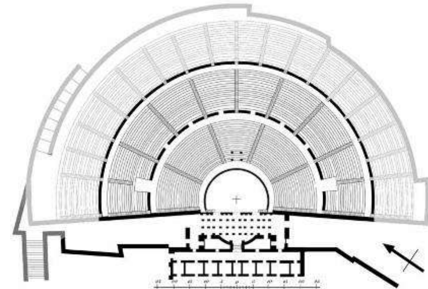
The Greco-Roman Theatre at Miletus - Plan View Note: Reconstruction Drawing of Roman Theatre - Shaded Upper Cavea Represents Missing Portions of Theatre Date of Construction: 3rd Century BC (Hellenistic) - 1st to mid 3rd Century AD (Roman) - Seating Capacity: (Hellenistic) - 5,300 (Roman) - 15,000 Theatron: 140m X 85 meters - 460m X 279 feet / Orchestra: 20m X 14 meters - 66m X 46 feet / Stage: 40m X 12 meters - 131m X 39 feet (Approximate measurements based on reconstruction drawing)
