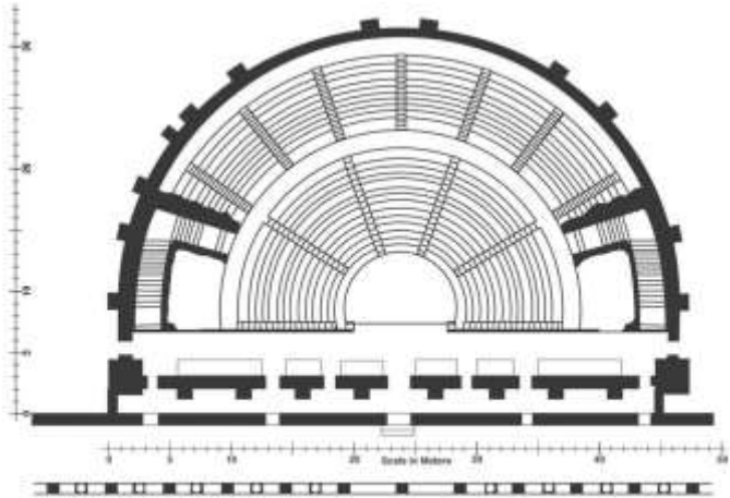
The Roman Odeion at Ephesus - Plan View Date of Construction: Circa 150 AD (Roman) Theatron: 47m X 22 meters - 154m X 125 feet - Orchestra: 36m X 5 meters - 30m X 16 feet - Stage: 30m X 4 meters - 98m X 13 feet
