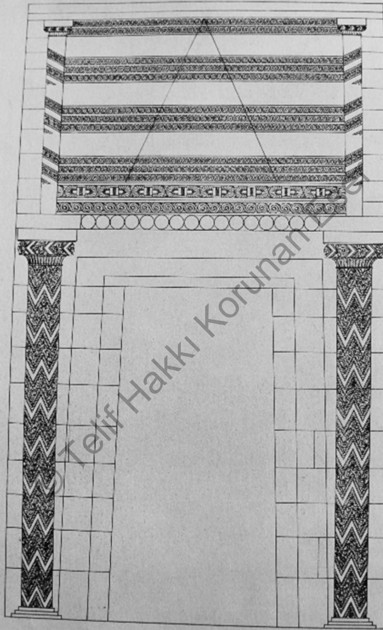
51. TREASURY OF ATREUS, façade, tentative reconstruction, scale about 1:50
