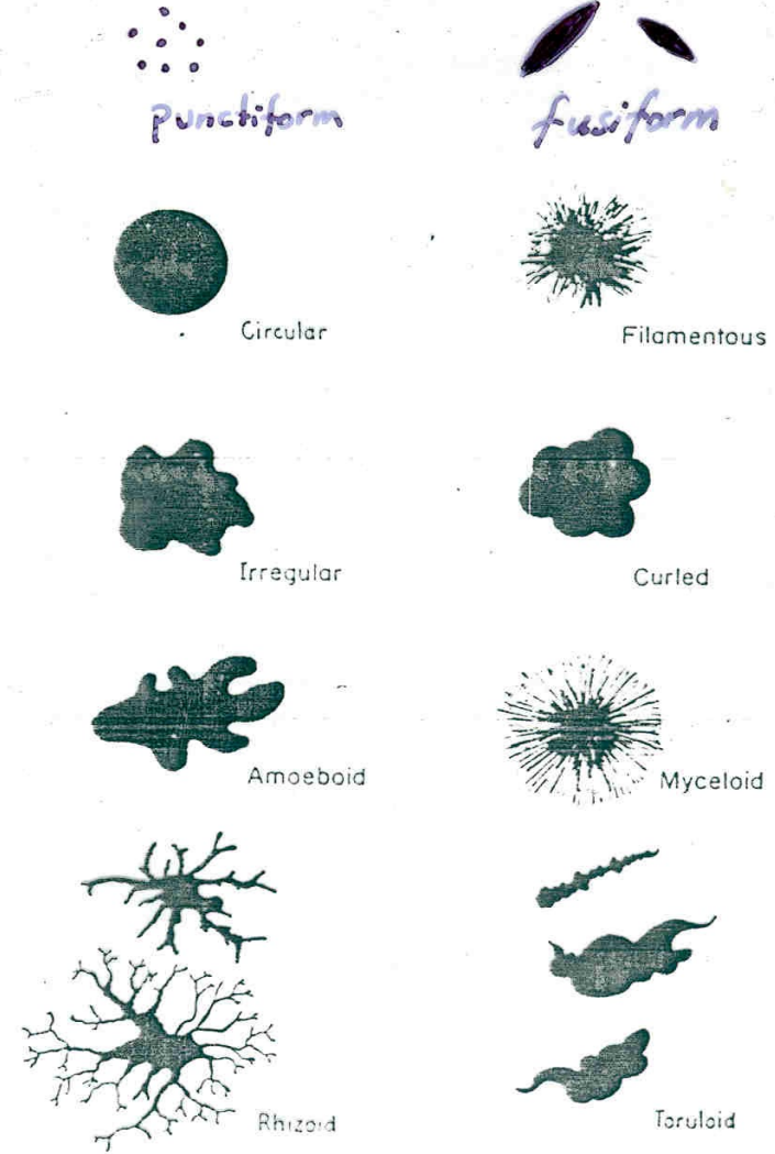
FIG. 124. Shape or form of colonies.
