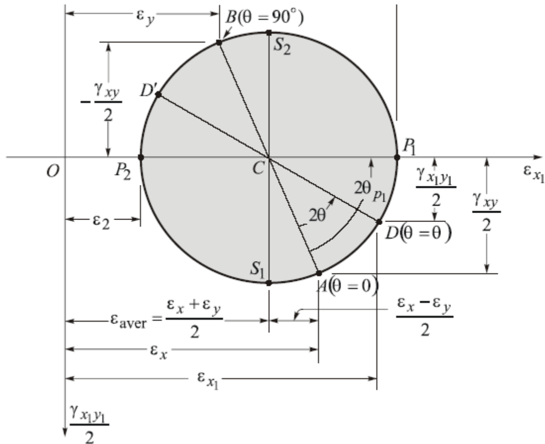
Fig. 5.6 Mohr's circle for plane strain
