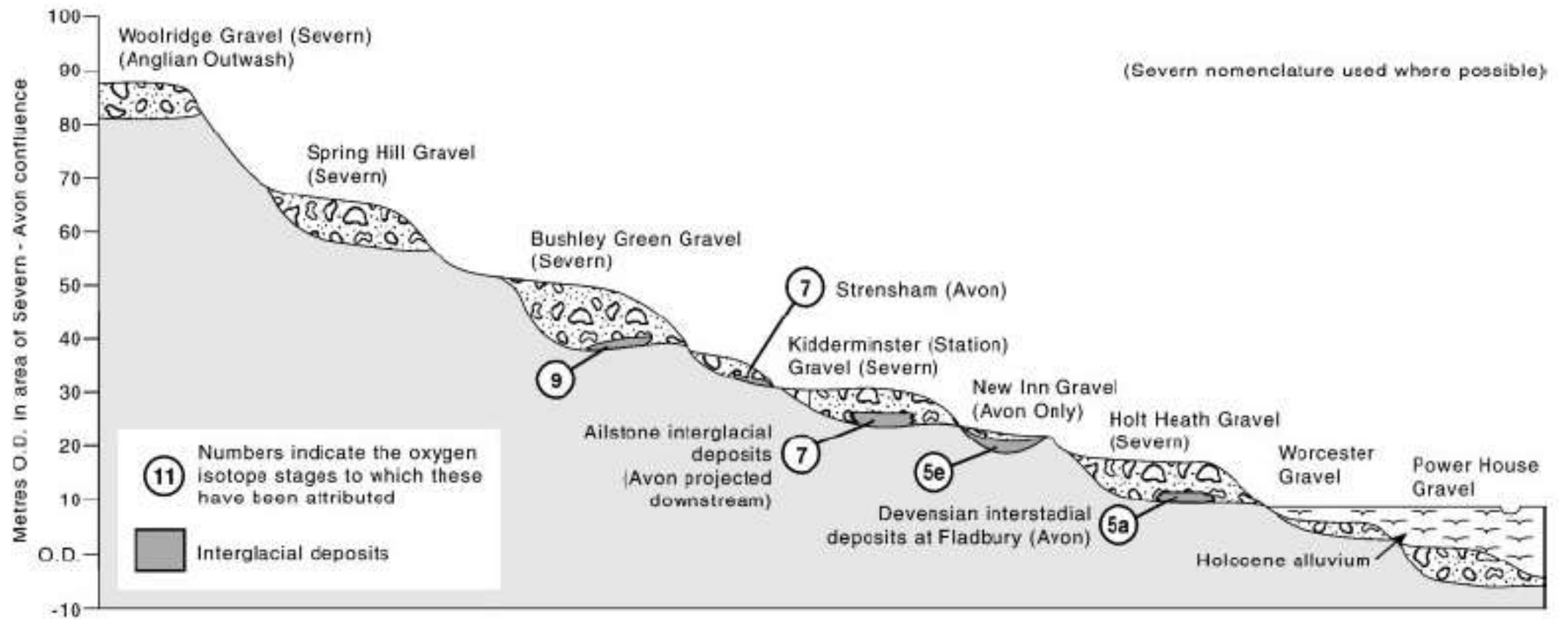
Figure 1 Idealised transect through the Severn–Avon terrace sequence. Severn nomenclature is applied where possible. Equivalent Avon units are shown in Table 1. Stratigraphical locations of amino acid data are indicated (see text)
