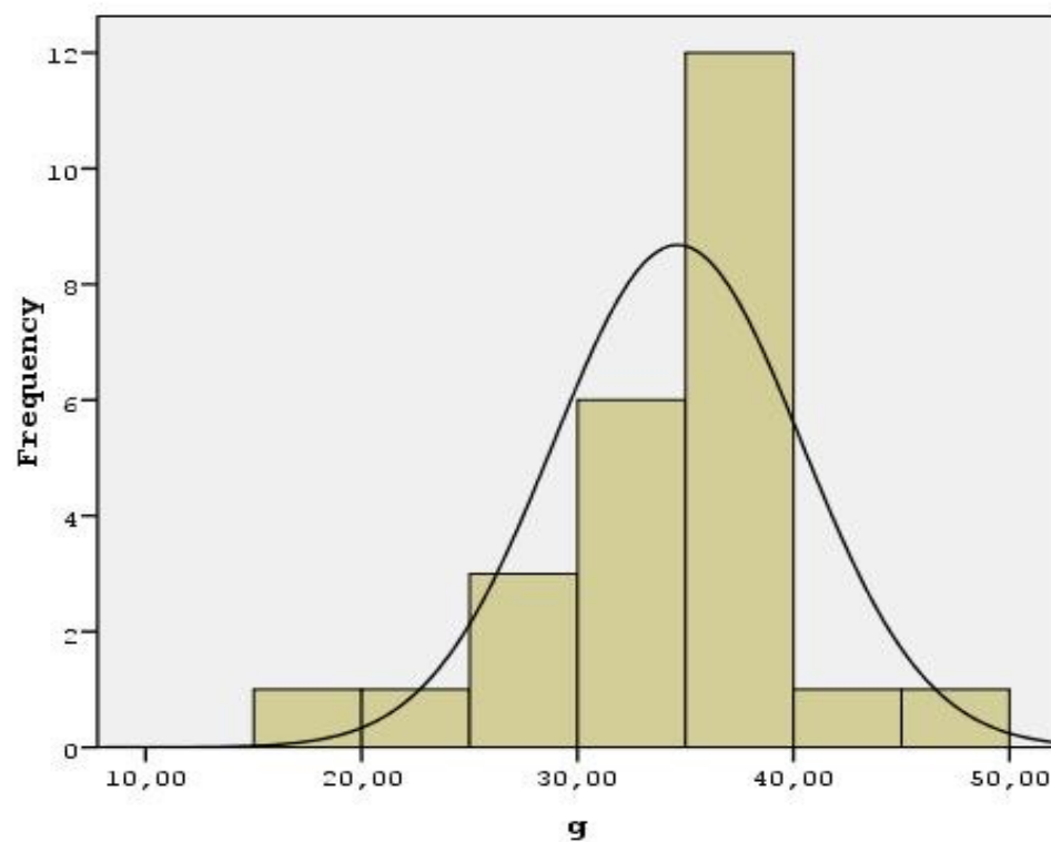
Histogram
