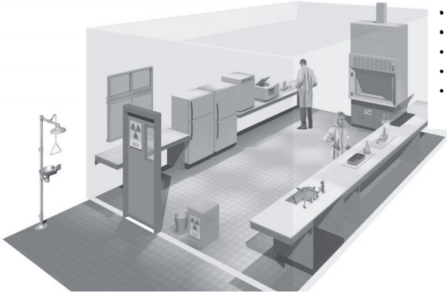
Figure 2. A typical Biosafety Level 1 laboratory (graphics kindly provided by CUH2A, Princeton, NJ, USA)
