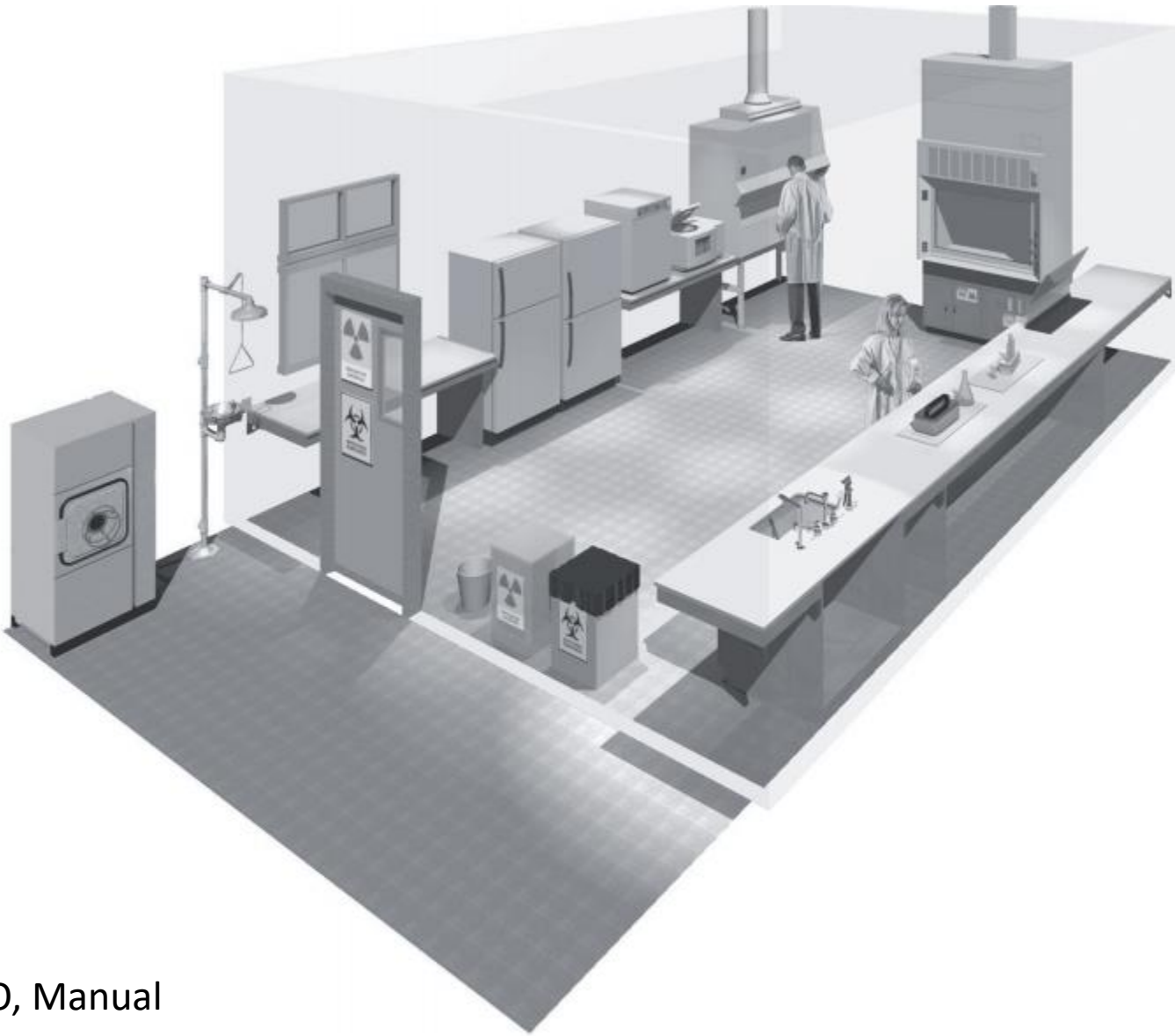
Figure 3. A typical Biosafety Level 2 laboratory
