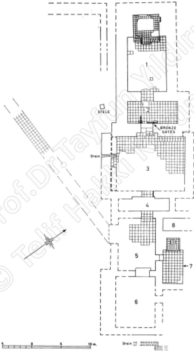
Plan of the Temple of Mamu at Balawat. Broken lines indicate probable wall alignments in unexcavated areas.
