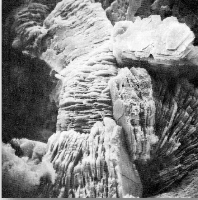
Kil mineralleri
