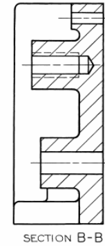
SECTION B-B
