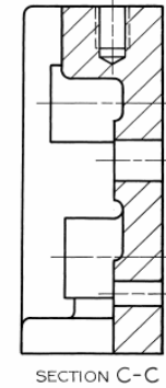
SECTION C-C
