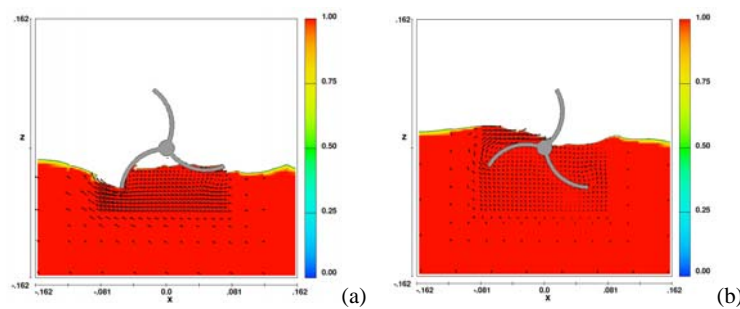
Fig. 4. Phase contours and local velocity vectors at t = 12.1 s; a) H = 100 mm; b) H = 160 mm
