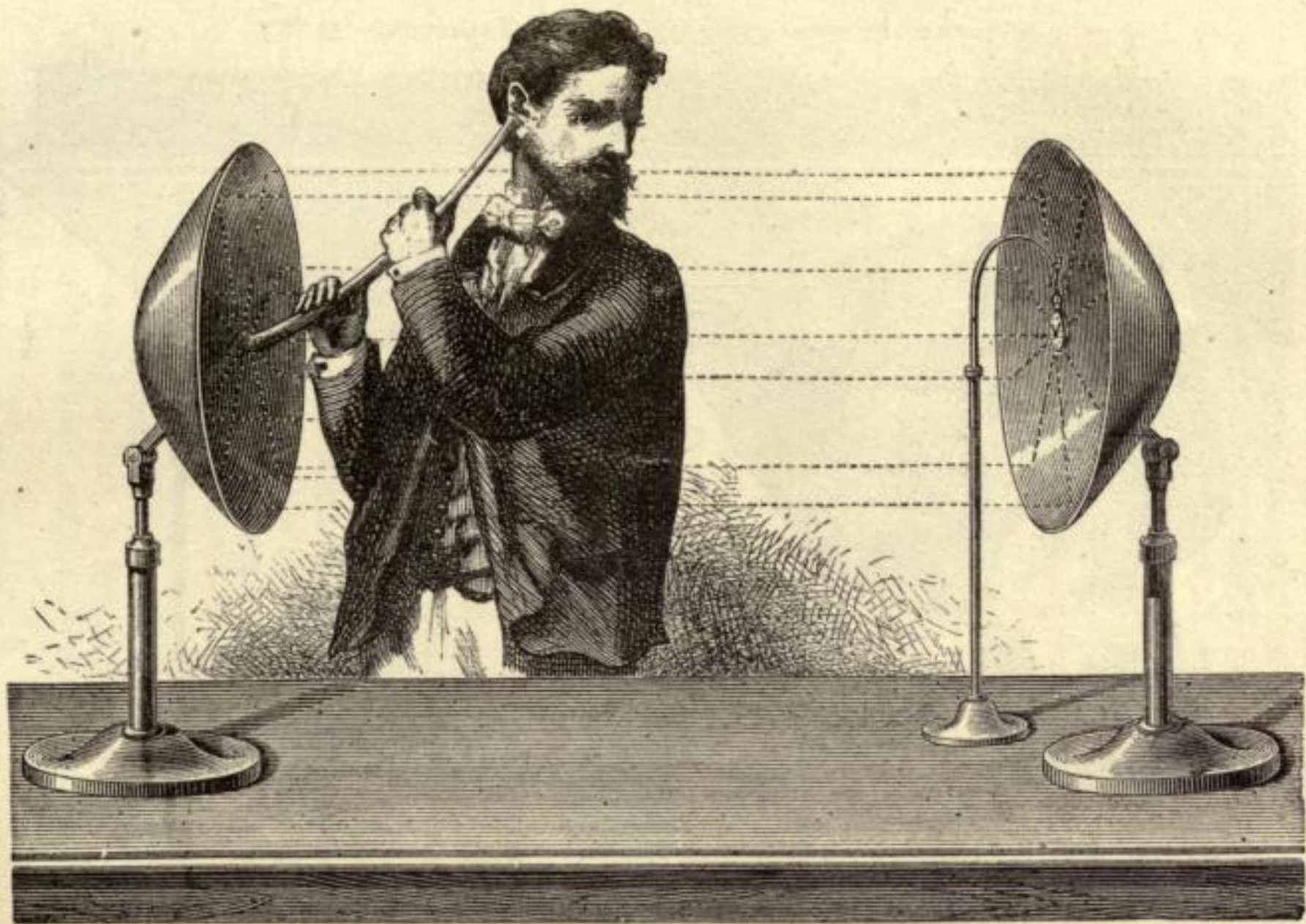
Fig. 26.—Experimental study of the laws of the reflection of sound.
