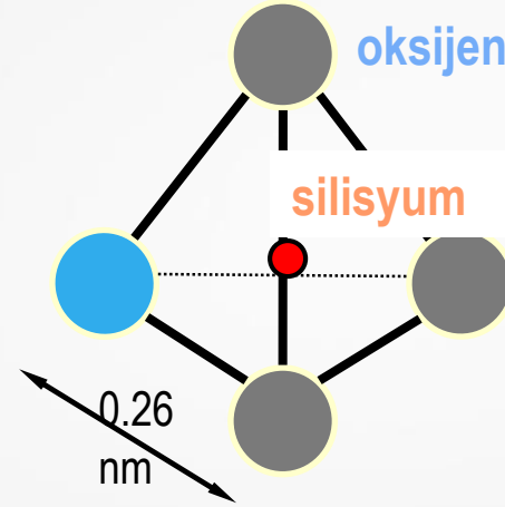
Silisyum tetraeder
