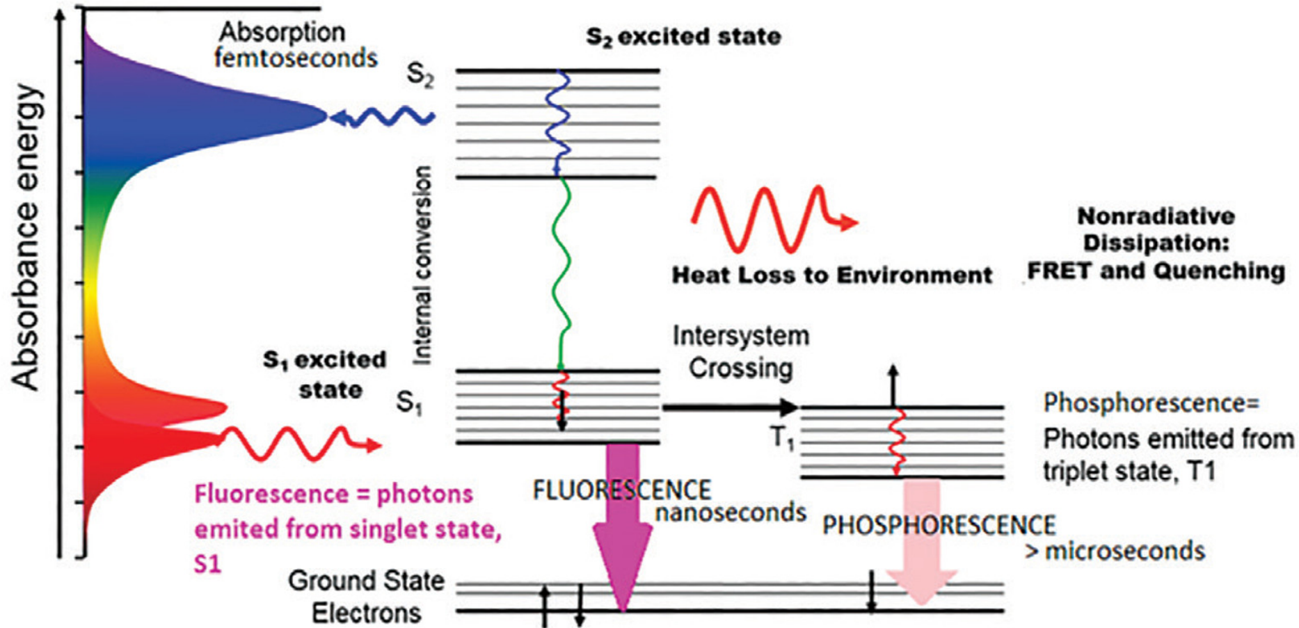
Jablonski Diagram for Fluorescence and Phosphorescence
