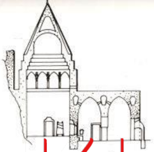
Fig. 3 Cross section A-B.
