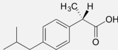
( S )-ibuprofen (active enantiomer)
