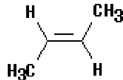
trans-2-butene (E)-2-butene
