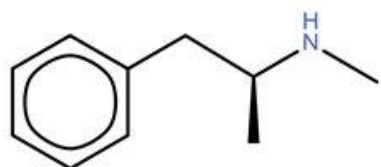
S methamphetamine (illegal psychotic drug)
