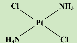
Transplatin
