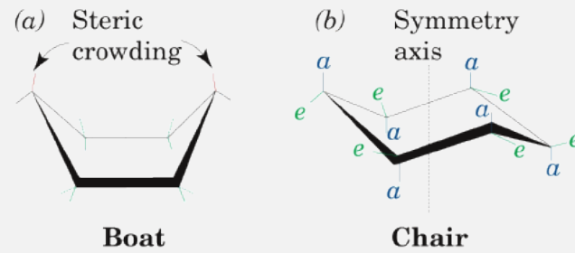
Conformations of the cyclohexane ring (a) in the boat conformation and (b) in the chair conformation
