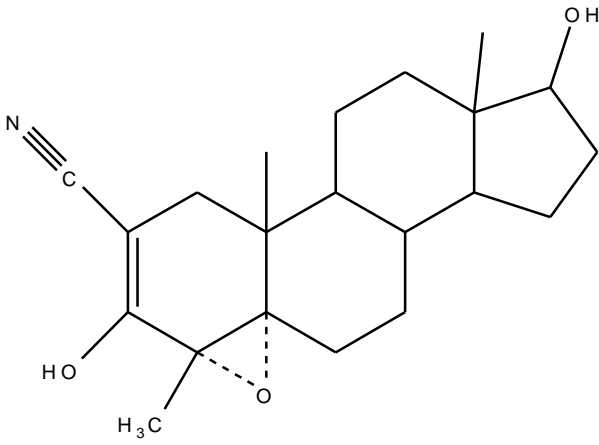
Trilostan
