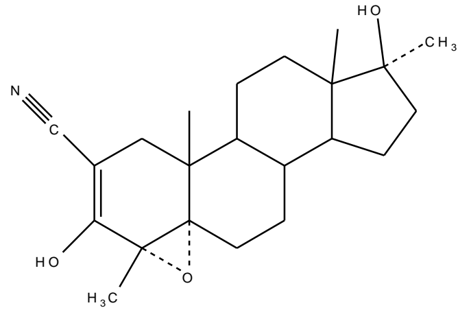
Epostan
